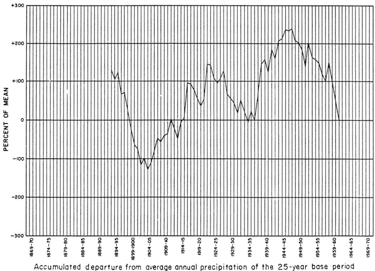
Figure 3. PRECIPITATION CHARACTERISTICS AT SQUIRREL INN NO.2
