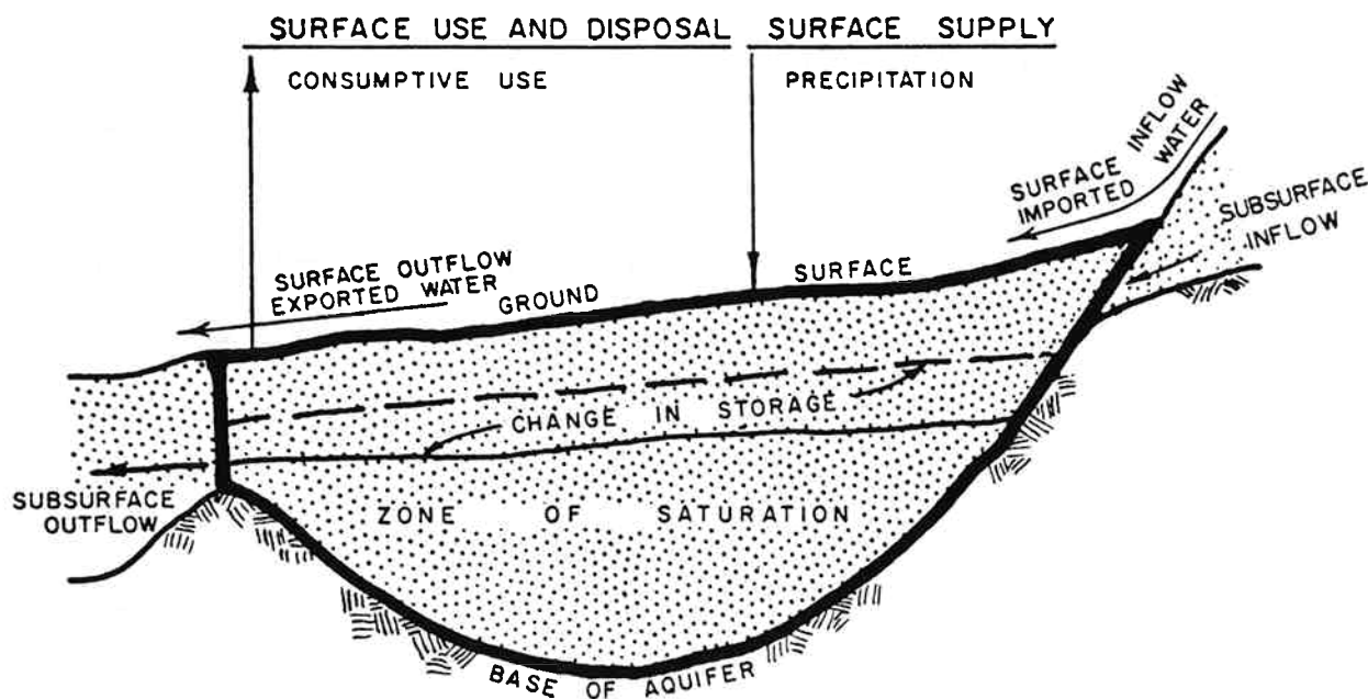
Fig. 6. THE GROUND WATER BASIN AS A FREE BODY
