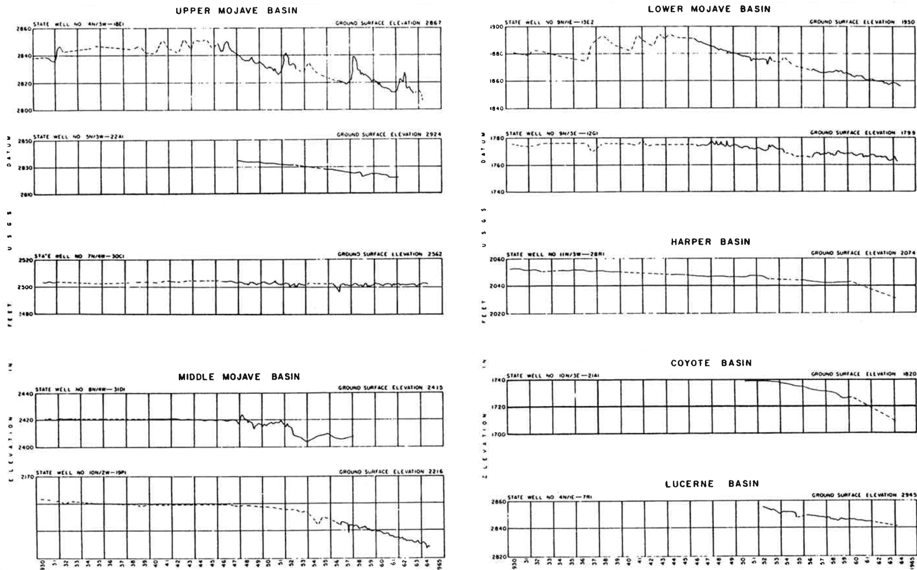
Figure 9. HYDROGRAPHS OF GROUND WATER AT REPRESENTATIVE WELLS
