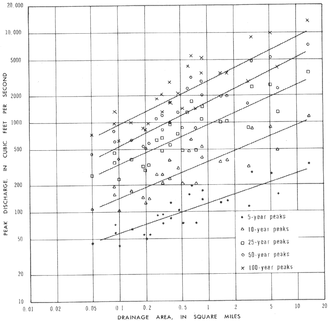
FIGURE 7.--Relation of discharge to drainage area for Lucerne Valley.
