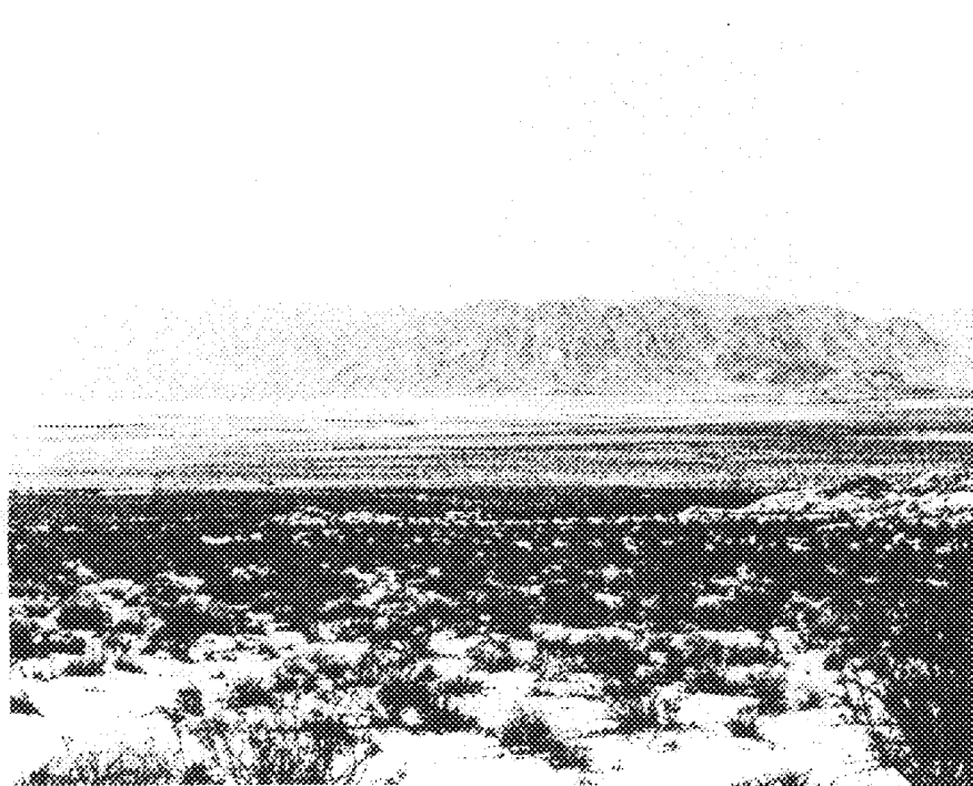
FIGURE 4.--View westward across north end of Lucerne Valley.
