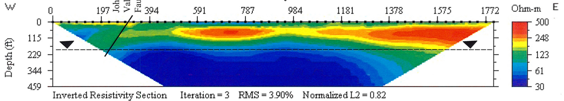
Figure 9 Resistivity Line 11
