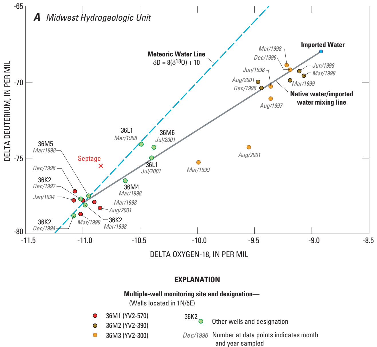
Figure 17. Stable isotopes from ground-water samples collected from selected wells in the (A) midwest and (B) mideast hydrogeologic units, Warren ground-water basin, San Bernardino County, California.
