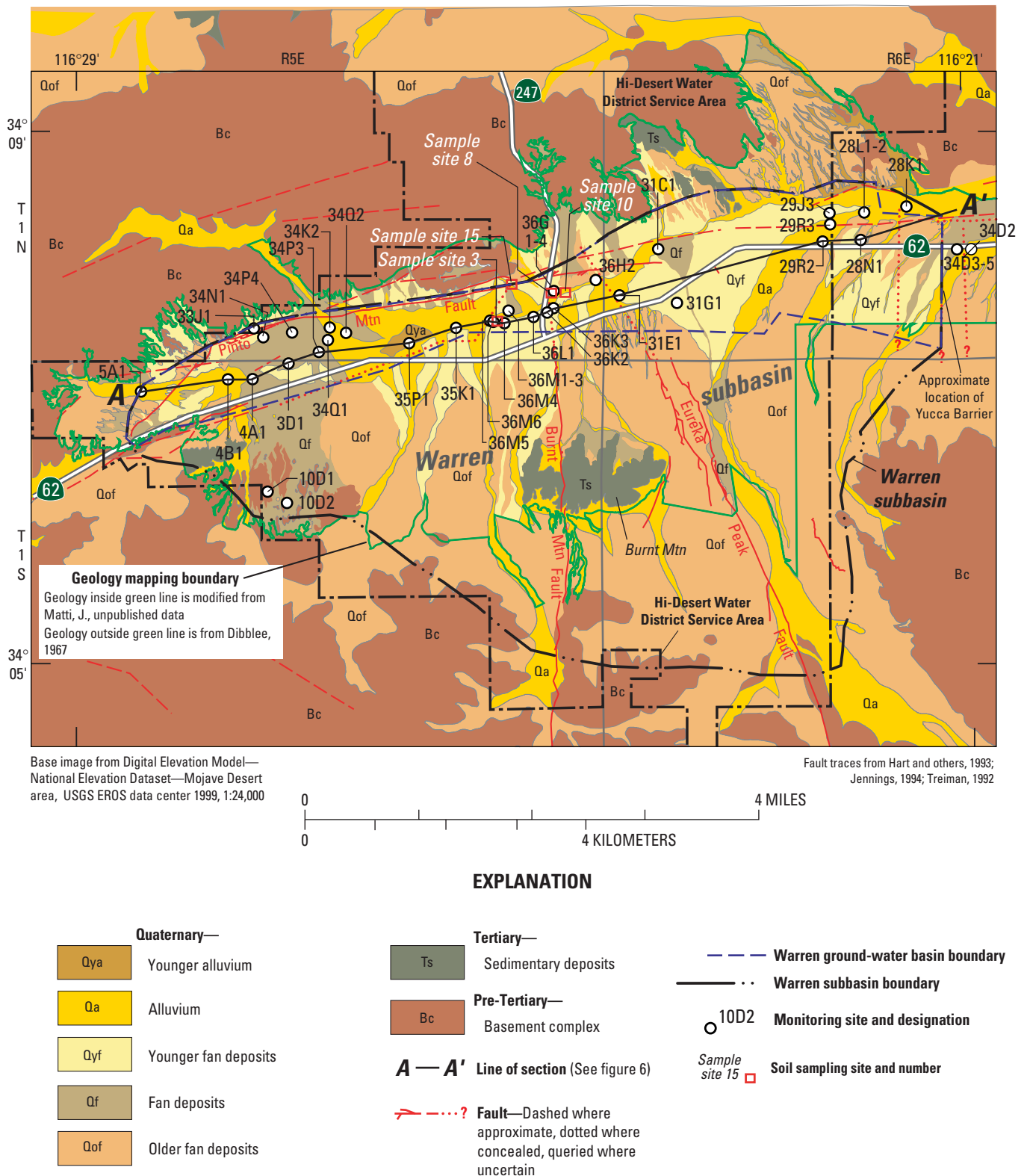
Figure 4. Generalized surficial geology, major faults, location of wells, and soil-sampling sites for the Warren subbasin, California.
