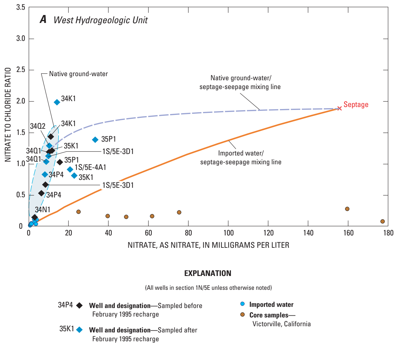
Figure 16. Relation between nitrate-to-chloride ratio and nitrate in ground-water samples from wells in the (A) west, (B) midwest, (C) mideast, and (D) northeast and east hydrogeologic units, Warren ground-water basin, San Bernardino County, California.
