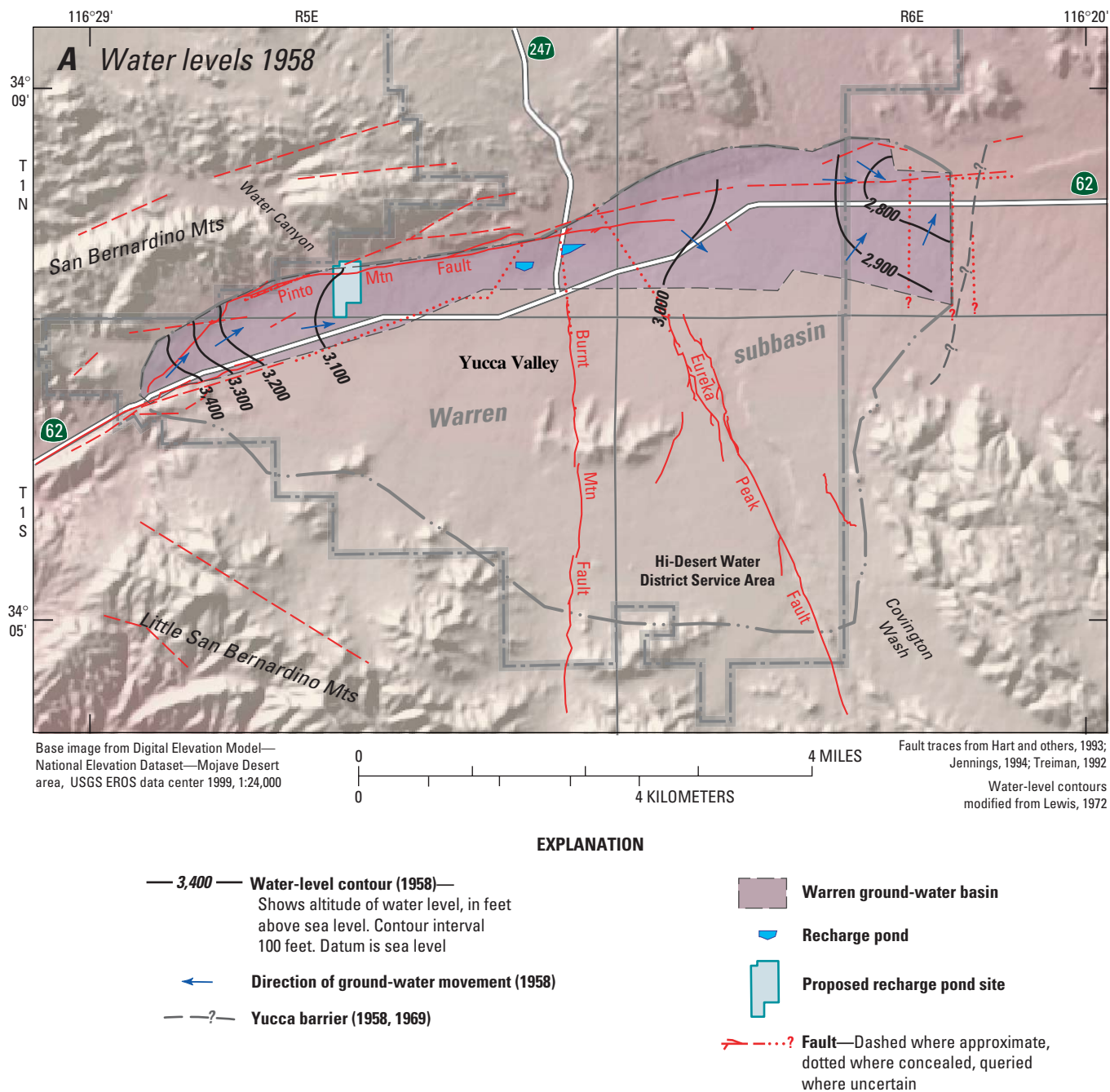
Figure 9. Water-level maps for (A) 1958, (B) 1969, (C) 1994, and (D) 1998, Warren ground-water basin, San Bernardino County, California.
