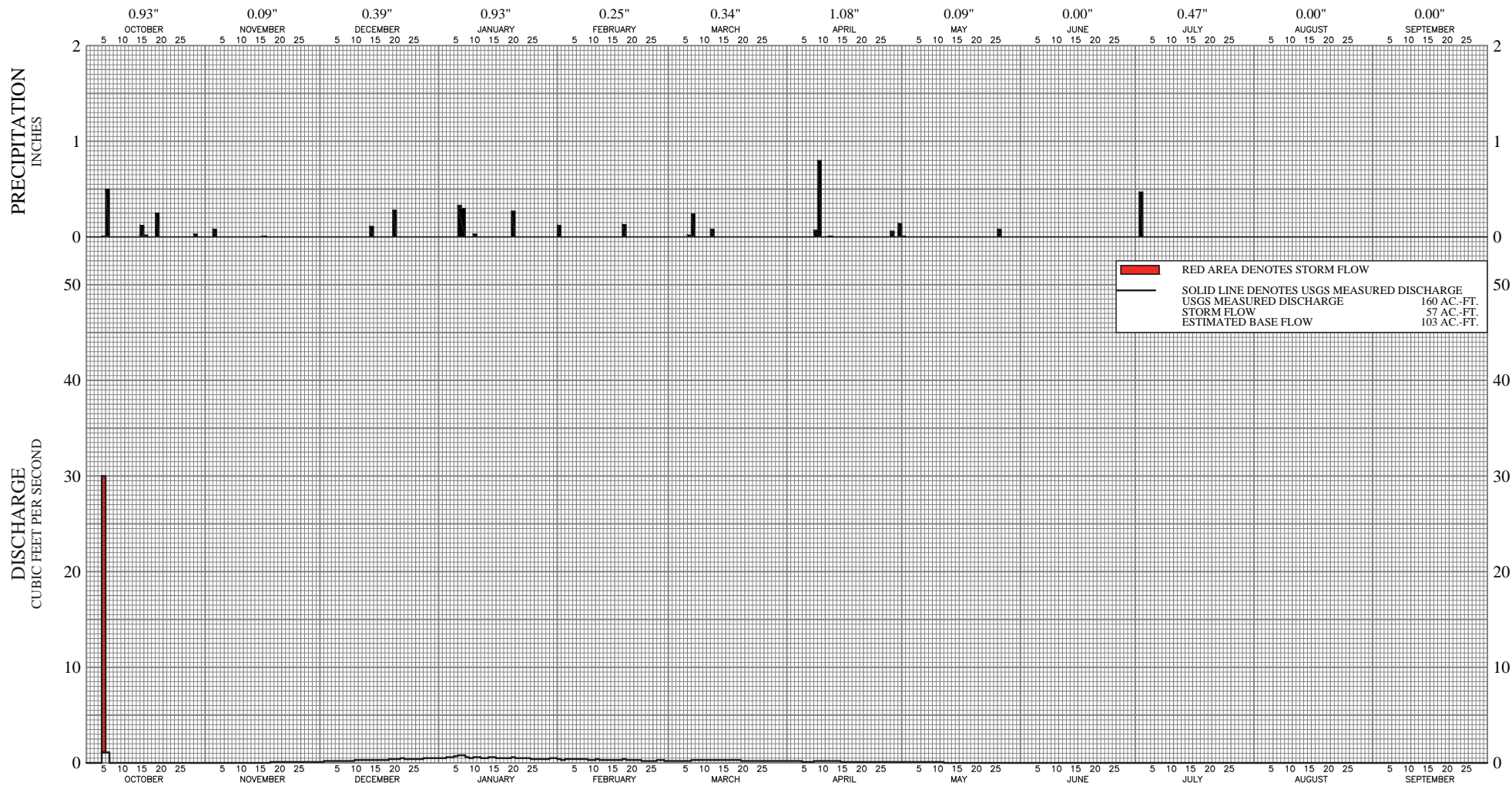
DISCHARGE OF MOJAVE RIVER AT AFTON AND PRECIPITATION AT BARSTOW WATER YEAR 2015-16
