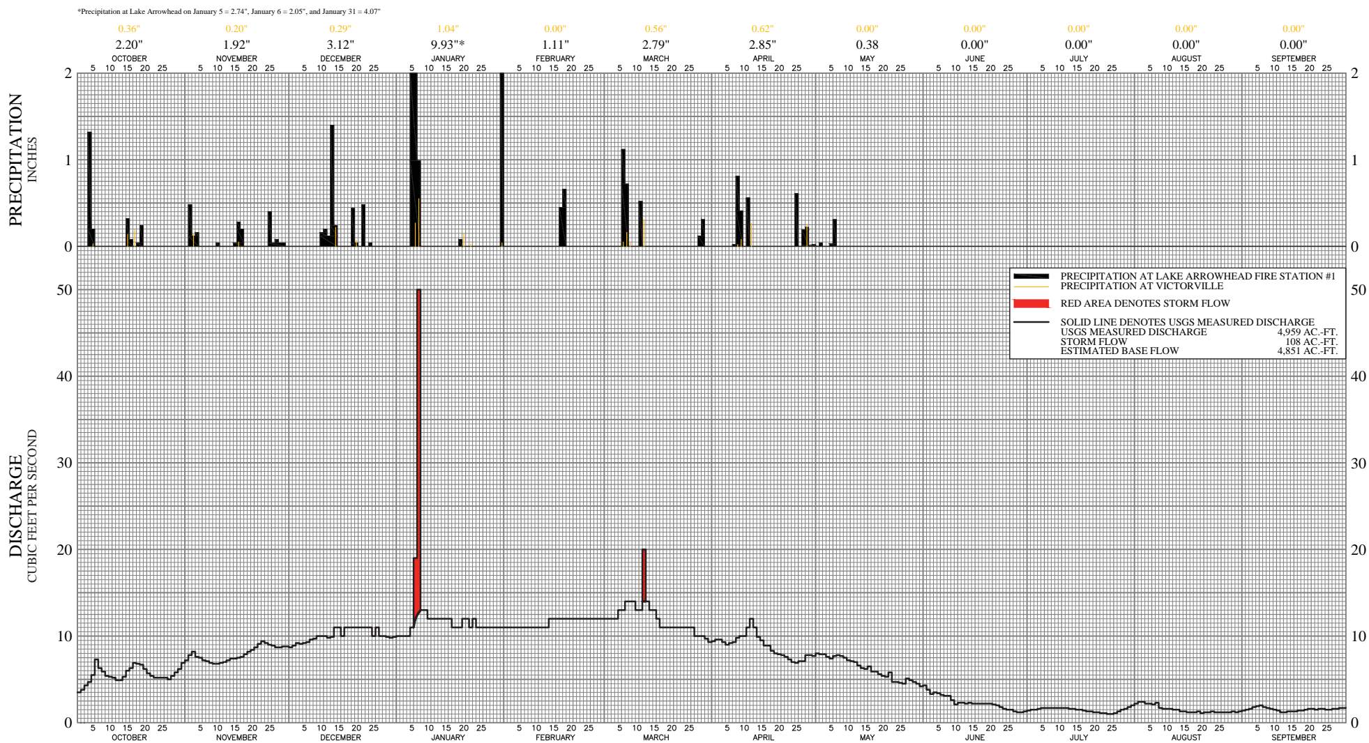
DISCHARGE OF MOJAVE RIVER AT LOWER NARROWS, PRECIPITATION AT LAKE ARROWHEAD FIRE STATION #1, AND PRECIPITATION AT VICTORVILLE WATER YEAR 2015-16
