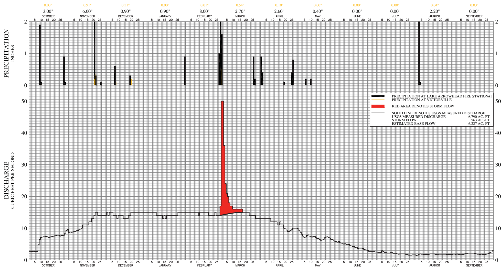
DISCHARGE OF MOJAVE RIVER AT LOWER NARROWS, PRECIPITATION AT LAKE ARROWHEAD FIRE STATION #1, AND PRECIPITATION AT VICTORVILLE WATER YEAR 2013-14
