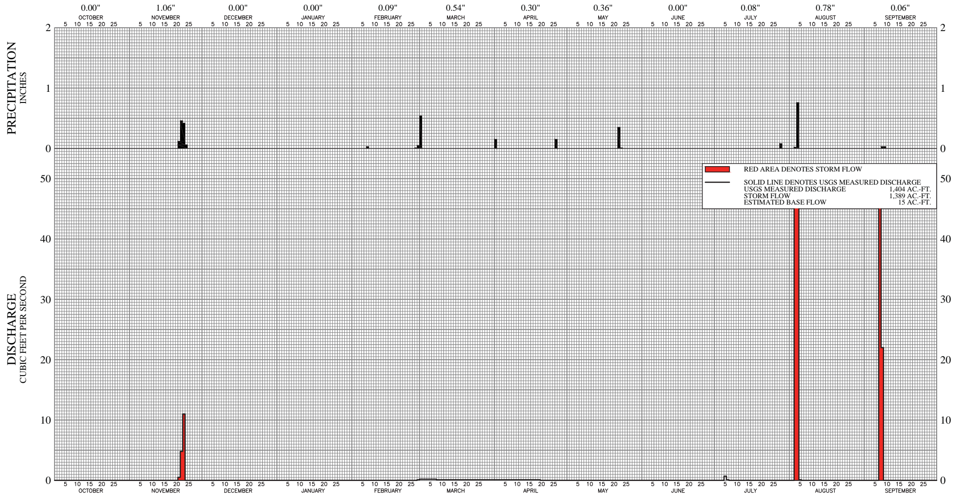
DISCHARGE OF MOJAVE RIVER AT AFTON AND PRECIPITATION AT BARSTOW WATER YEAR 2013-14
