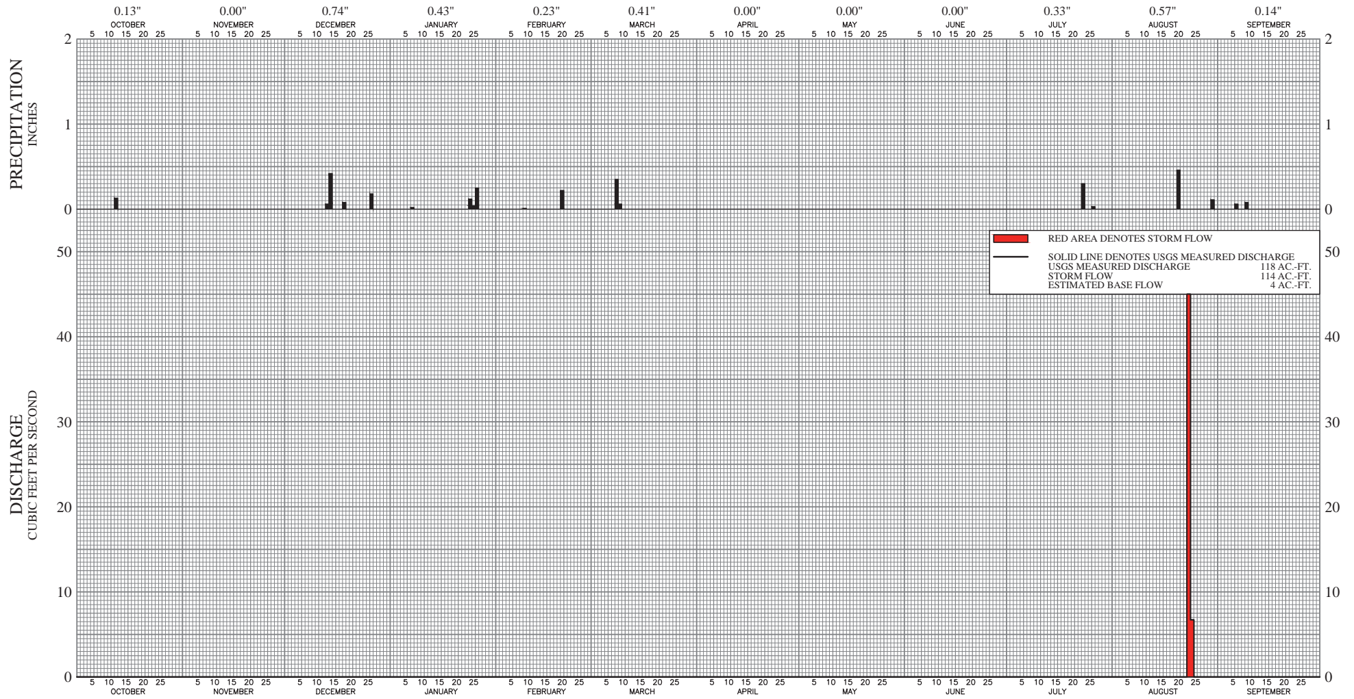
DISCHARGE OF MOJAVE RIVER AT AFTON AND PRECIPITATION AT BARSTOW WATER YEAR 2012-13
