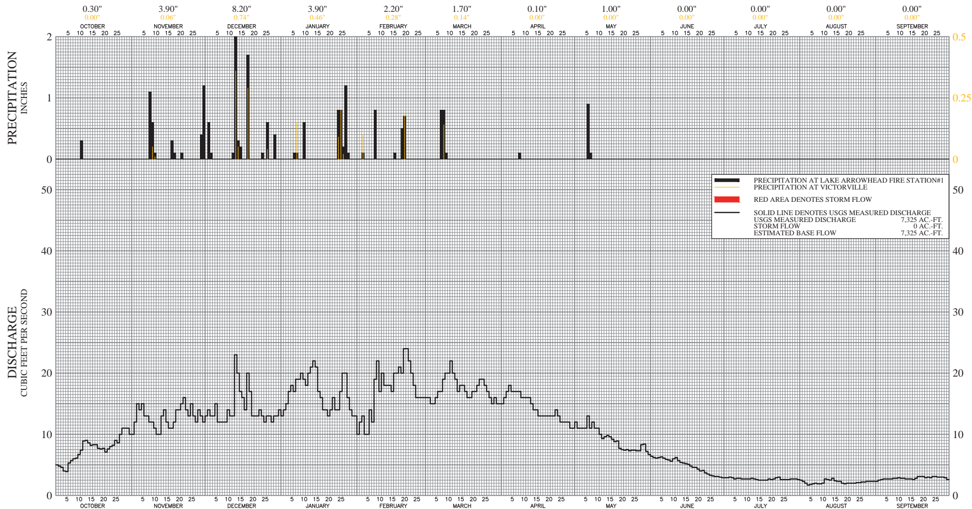
DISCHARGE OF MOJAVE RIVER AT LOWER NARROWS, PRECIPITATION AT LAKE ARROWHEAD FIRE STATION #1, AND PRECIPITATION AT VICTORVILLE WATER YEAR 2012-13
