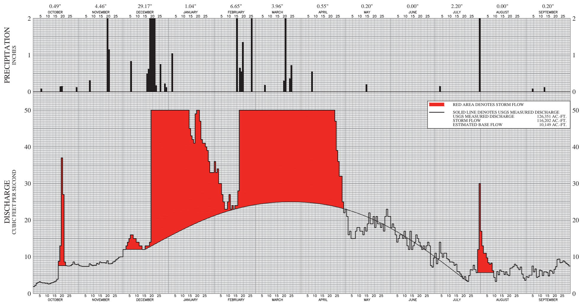
DISCHARGE OF MOJAVE RIVER AT LOWER NARROWS AND PRECIPITATION AT LAKE ARROWHEAD FIRE STATION #2 WATER YEAR 2010-11
