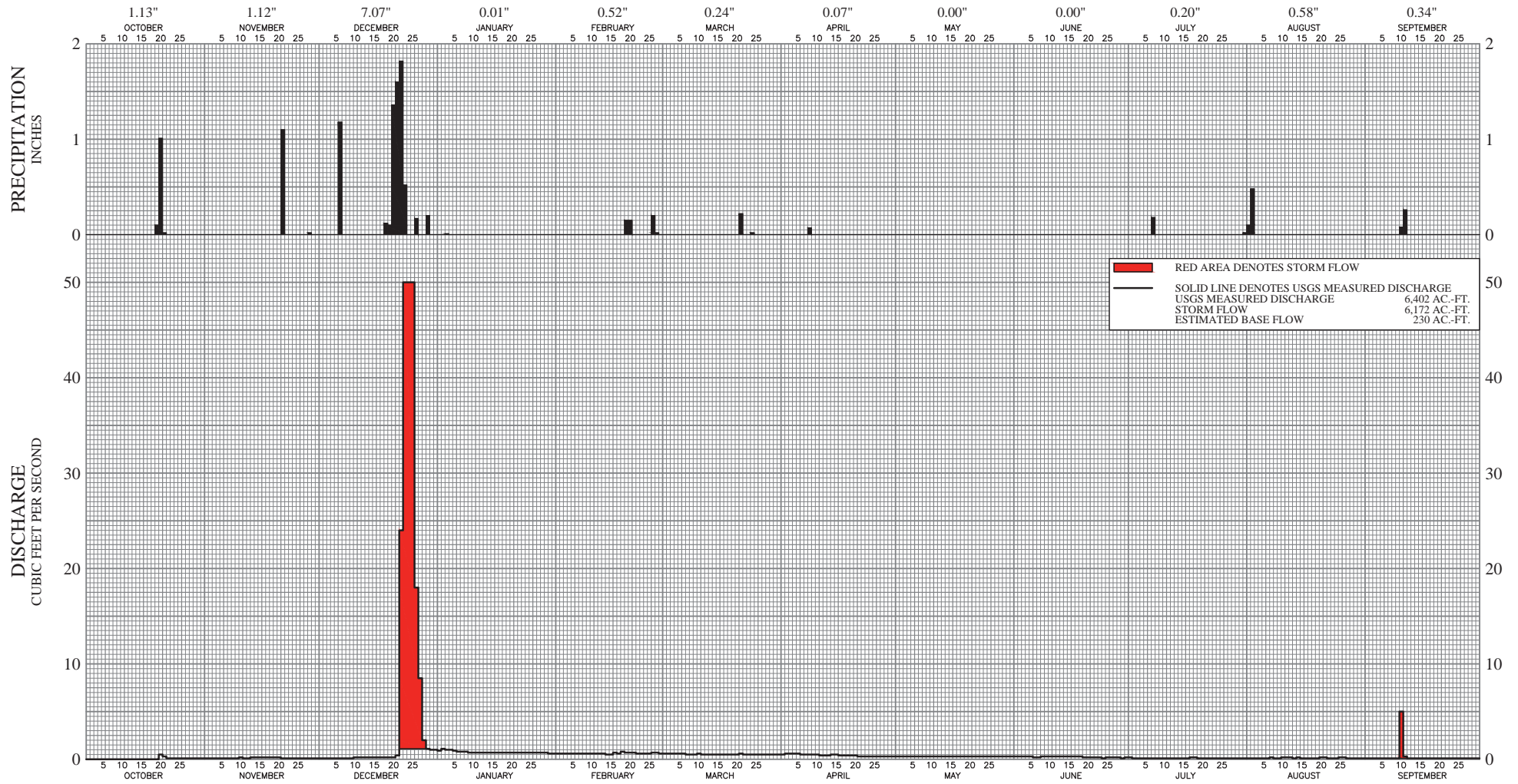
DISCHARGE OF MOJAVE RIVER AT AFTON AND PRECIPITATION AT BARSTOW WATER YEAR 2010-11
