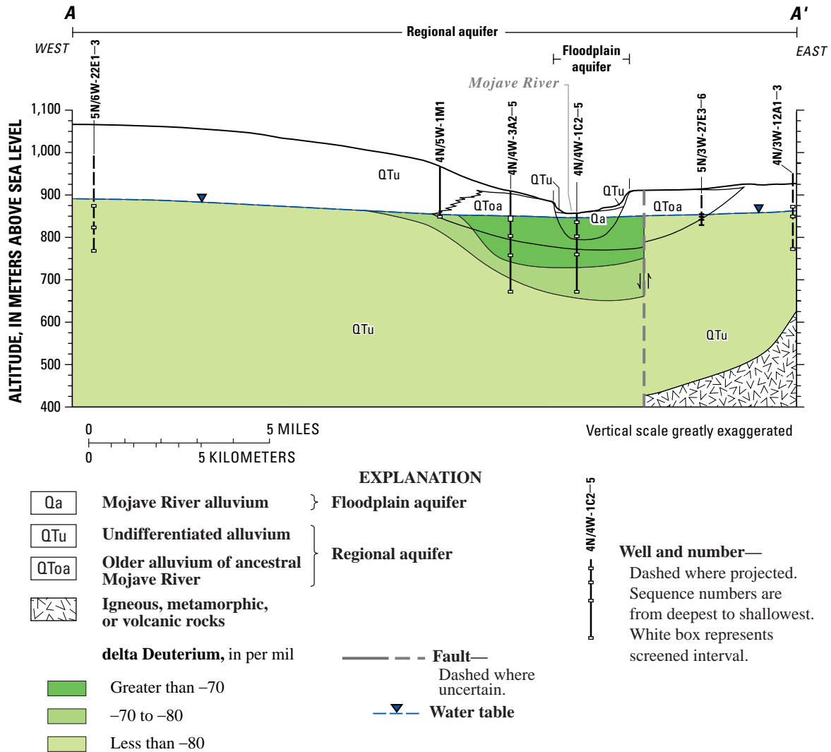
Figure 7. Delta deuterium composition of water from selected observation wells along section A–A', Mojave River ground-water basin, southern California. See figure 1 for location of sections. (Modified from Stamos and others, 2001.)
