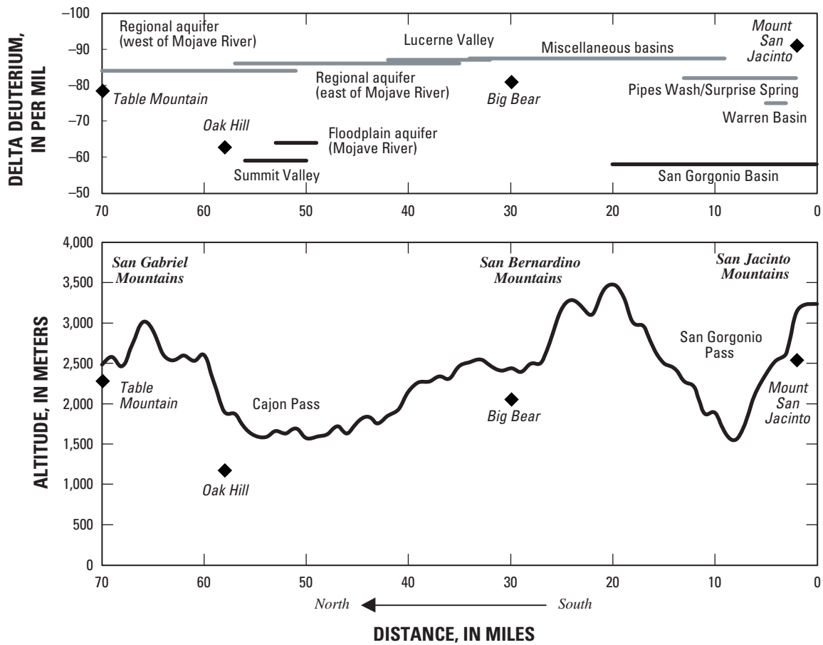
Figure 3. Altitude along topographic divide and changes in delta deuterium composition of ground water on the eastern slope of the San Gabriel, the San Bernardino, and the San Jacinto Mountains, southern California. (Median delta deuterium composition of ground water and extent along mountain front shown as gray bars)
