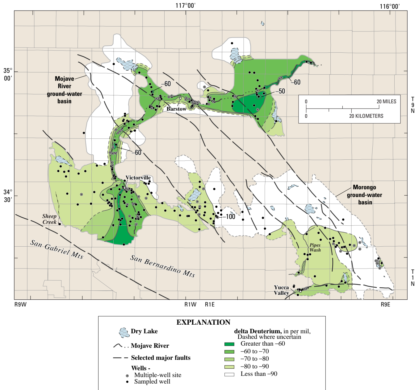
Figure 5. Delta deuterium composition of water from wells in the Mojave River and the Morongo ground-water basins, southern California, 1986–2000.
