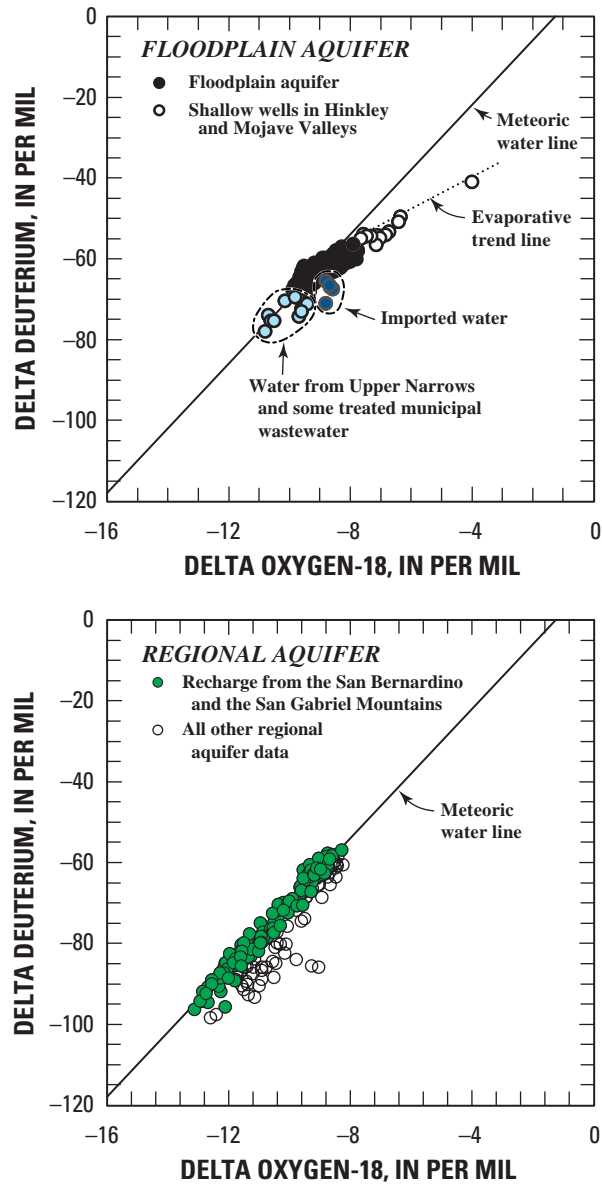
Figure 6. Delta oxygen-18 and delta deuterium composition of water from wells in the floodplain aquifer and the regional aquifer of the Mojave River ground-water basin, southern California, 1986–2000.
